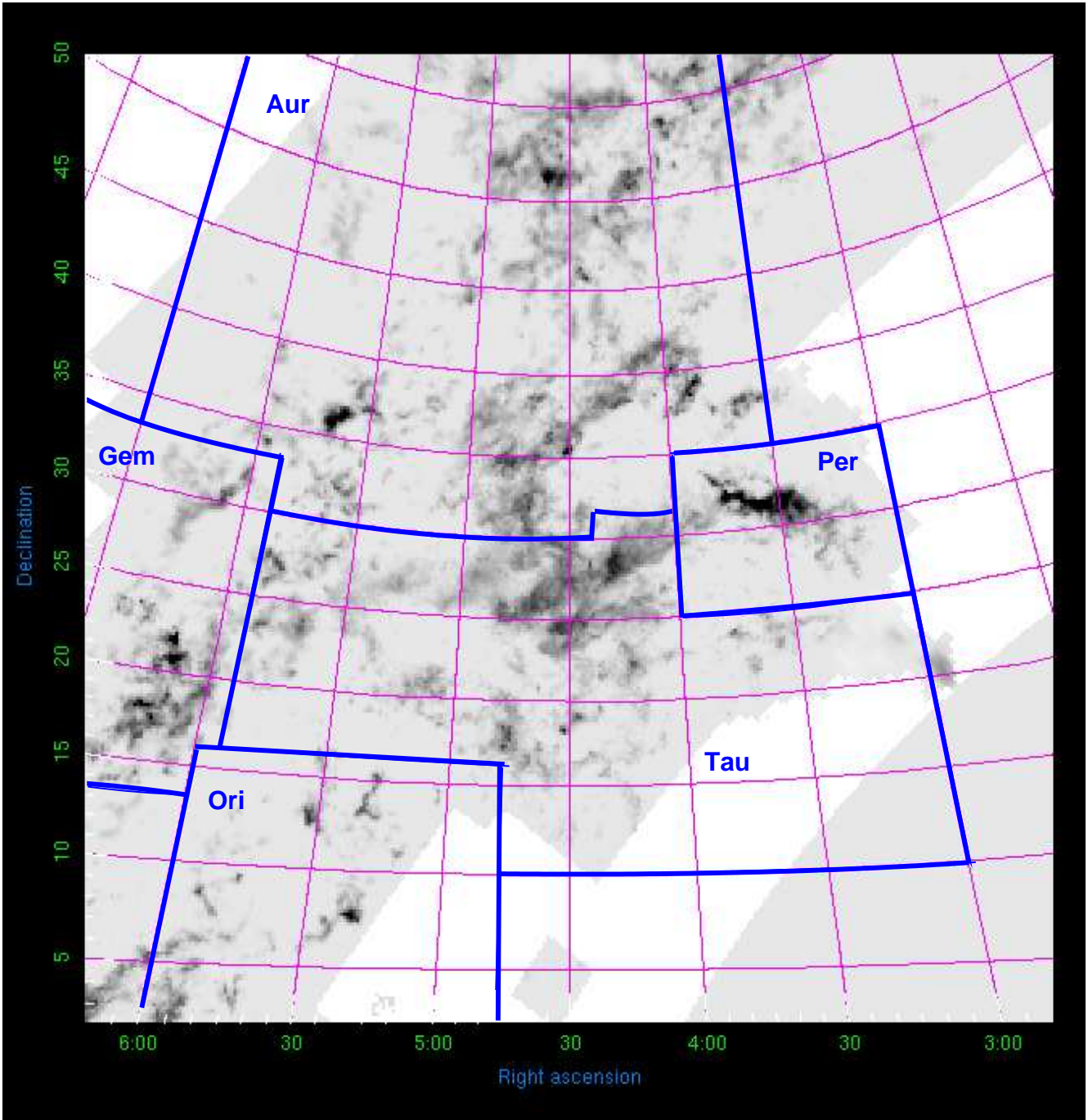
Figure 2: Perseus, Taurus, Auriga, Orion
