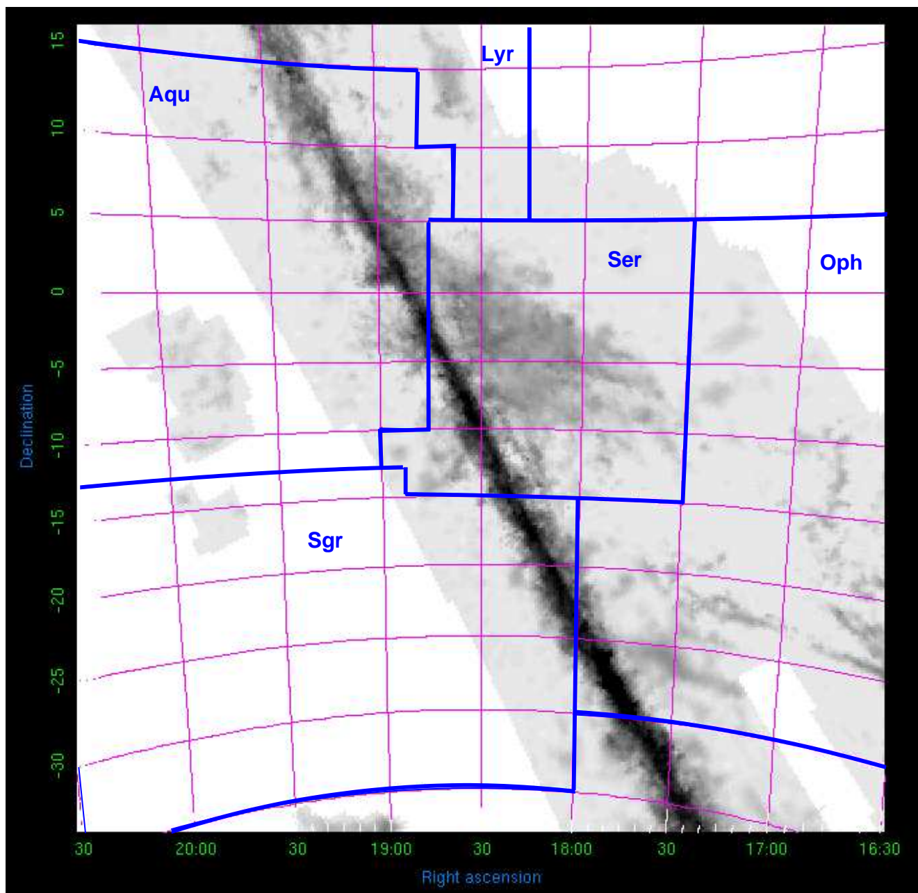
Figure 7: Ophiuchus, Sagittarius, Serpens, Aquilla, Lyra
