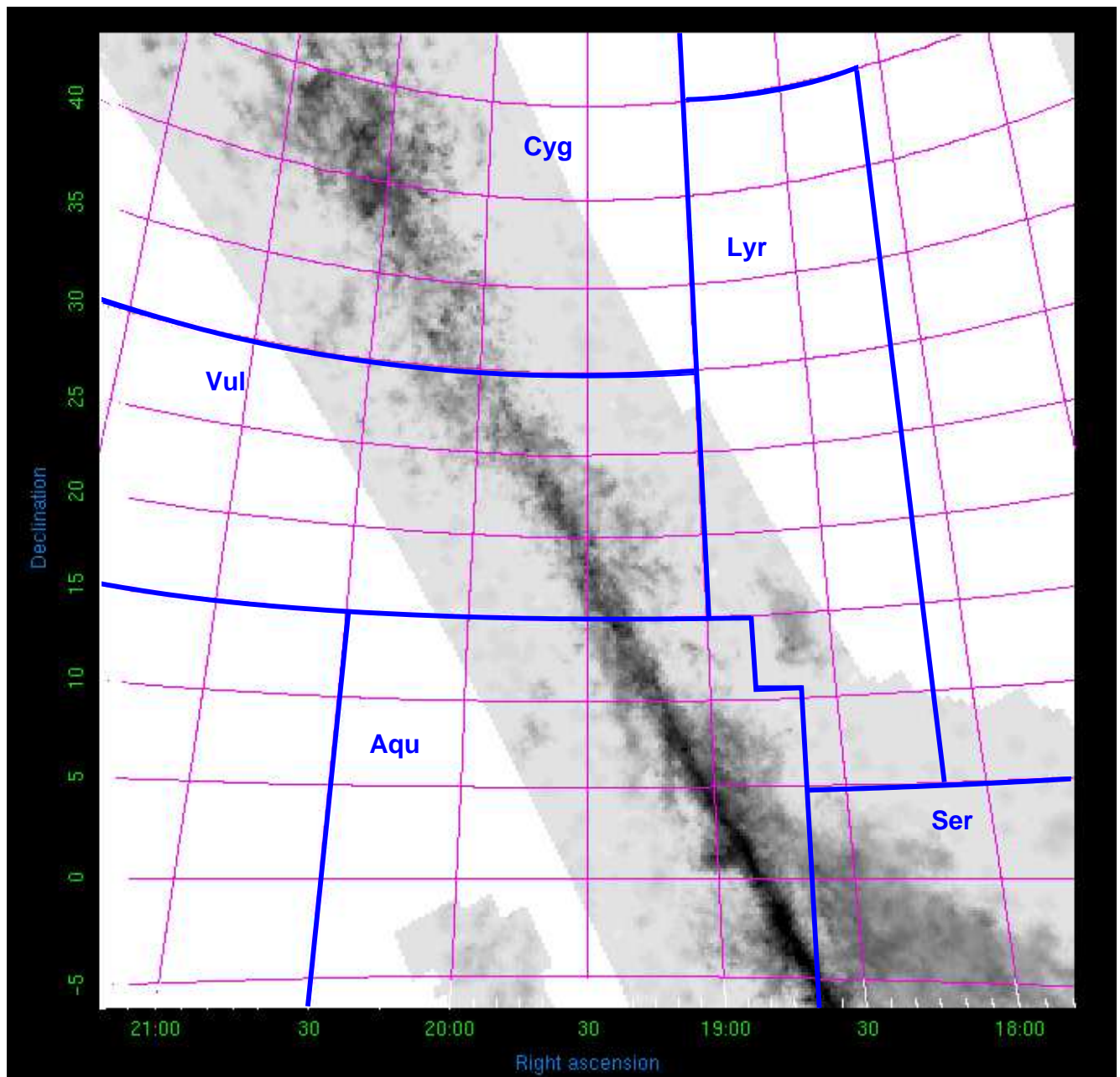
Figure 8: Serpens, Aquilla, Lyra, Vulpecula, Cygnus
