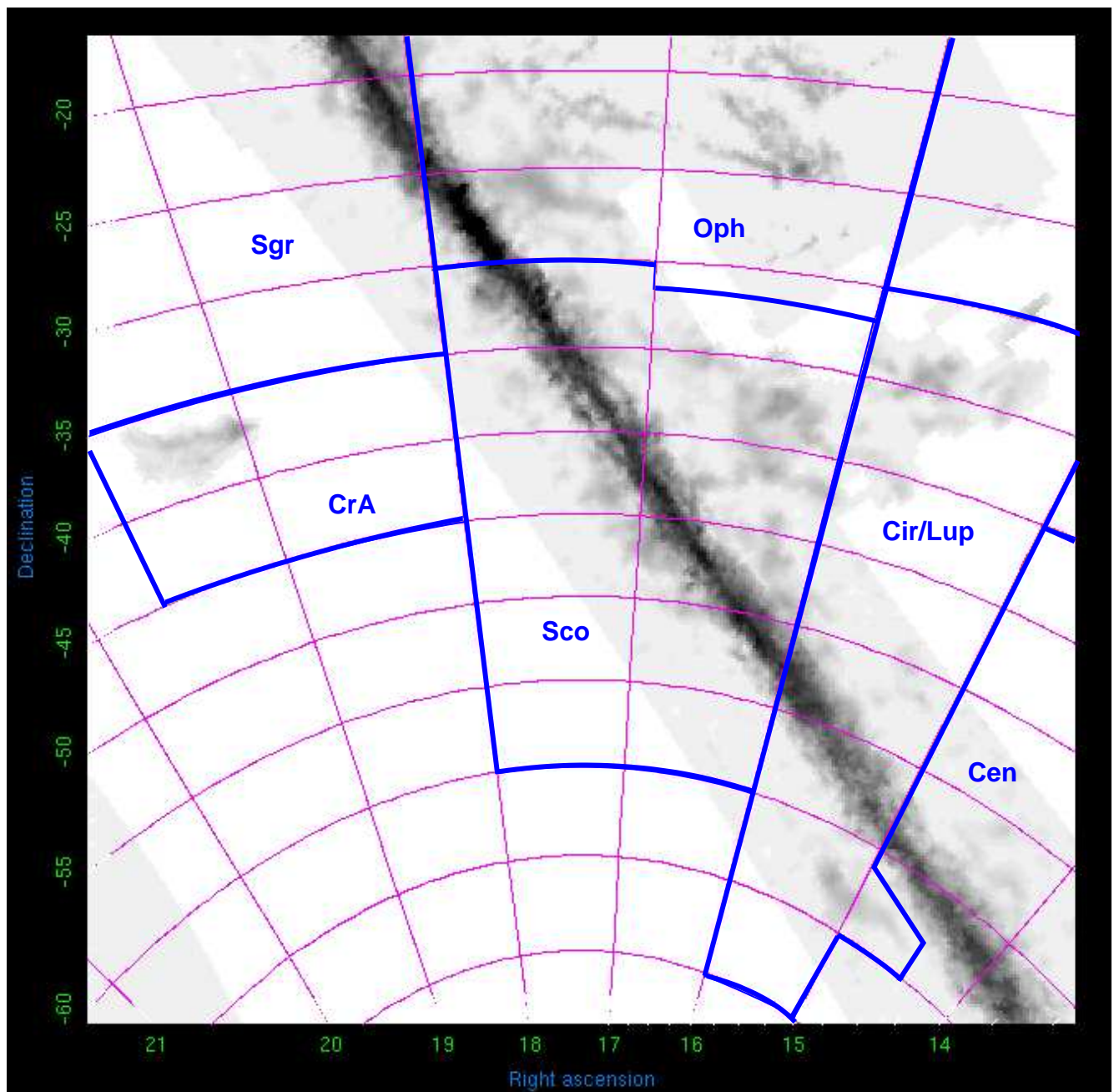
Figure 6: Circinus/Lupus, Scorpius, Corona Australis, Ophiuchus, Sagittarius
