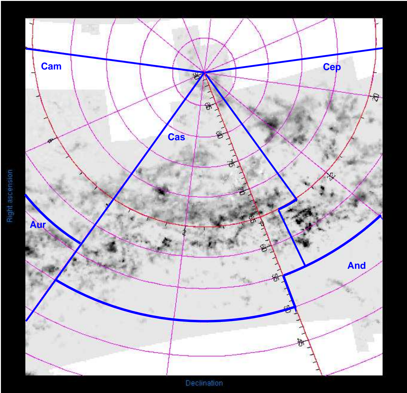
Figure 1: Cepheus, Cassiopeia, Camelopardalis
