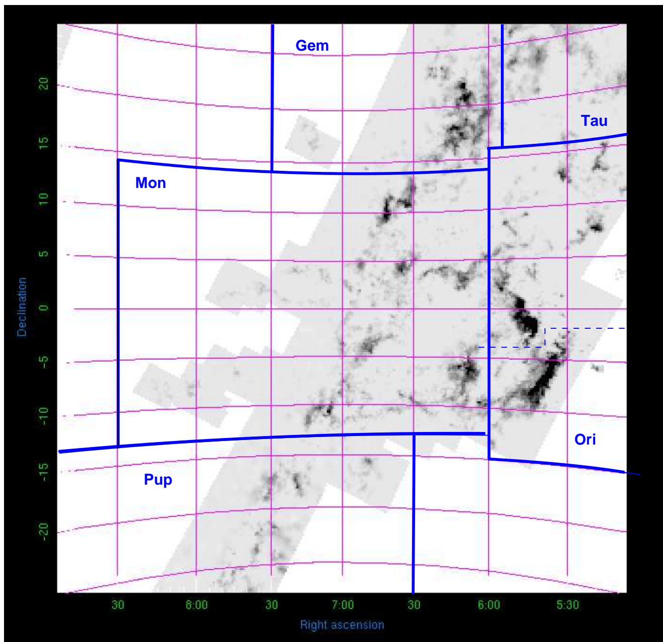
Figure 3: Orion, Monoceros, Taurus, Gemini, Puppis
