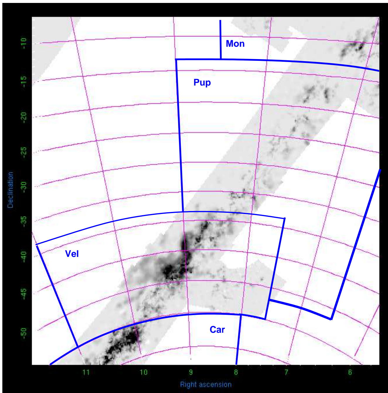
Figure 4: Puppis, Vela, Carina
