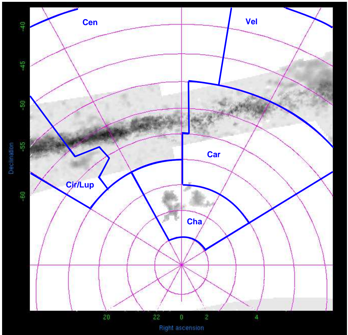
Figure 5: Vela, Carina, Chameleon, Centaurus, Circinus/Lupus
