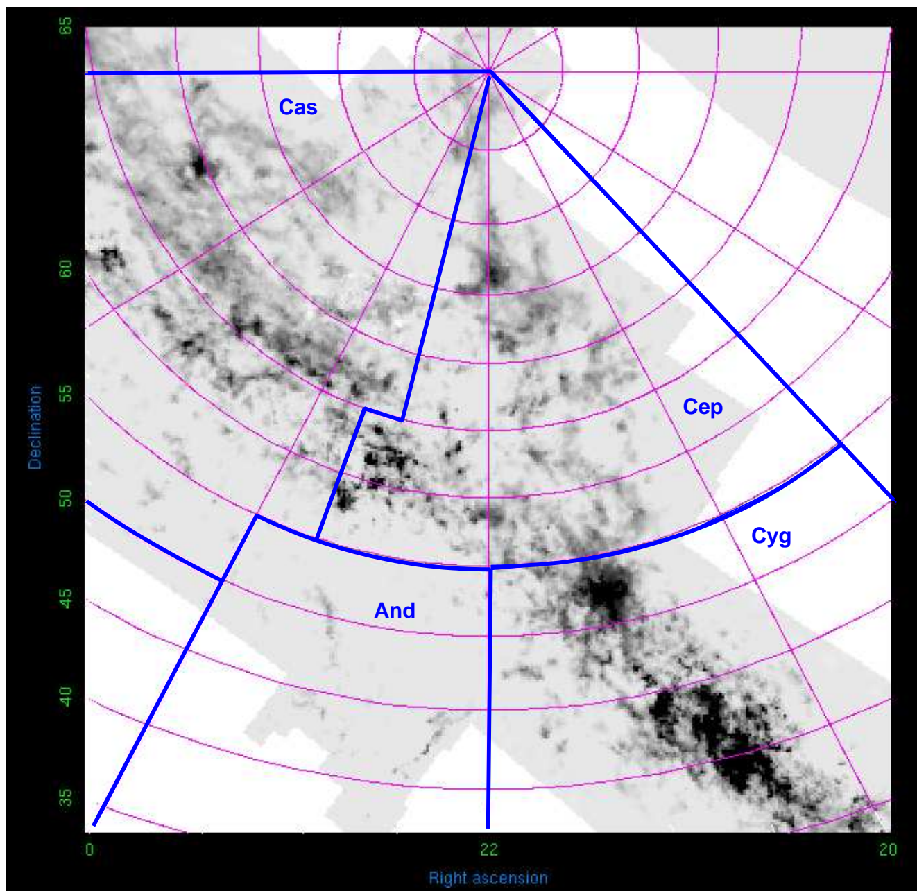
Figure 9: Cygnus, Andromeda, Cepheus, Cassiopeia
